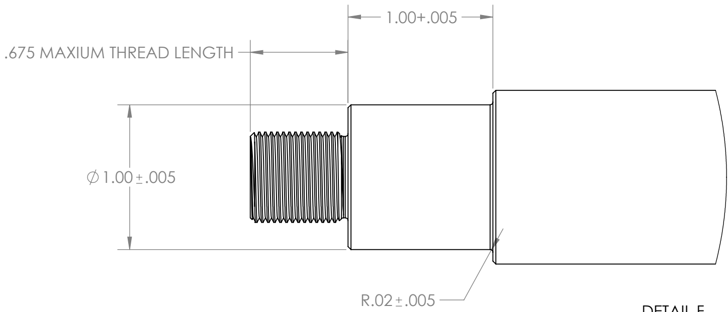
DETAIL F SCALE 1.5 : 1
